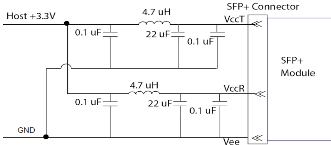
Figure2. Host Board Power Supply Filters Circuit
