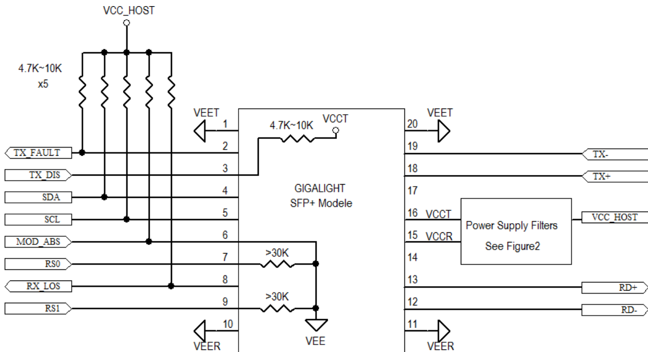
Figure3. Host-Module Interface
