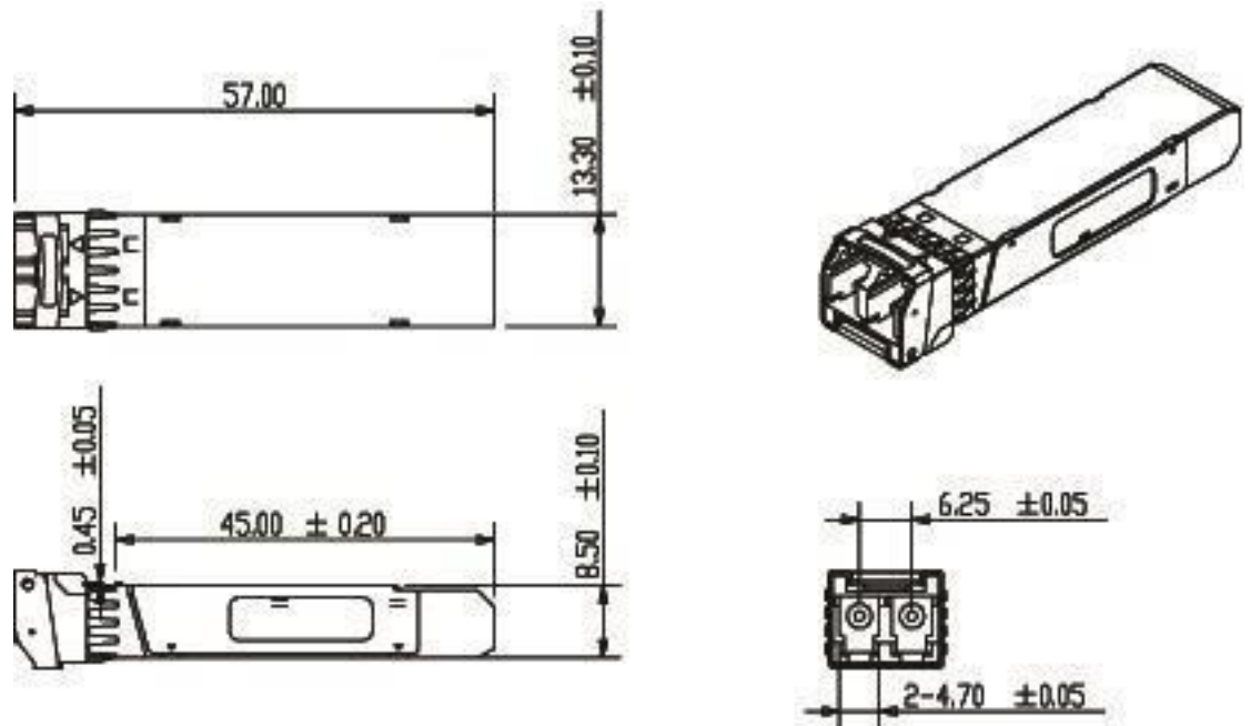
Figure6. Mechanical Specifications
